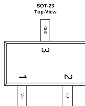
Figure.1 Pin Configuration & Functions
